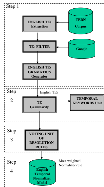
Figure 3. Automatic assignment of resolution rules
