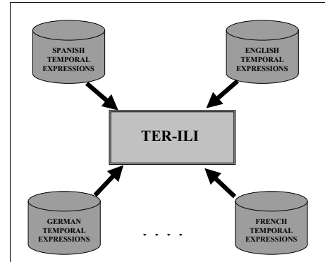
Figure 1. Multilingual TERSEO
